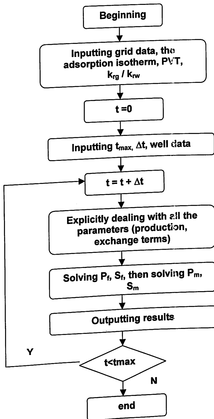
Fig 4.1:- The Flow Chart of Simulator Calculation
