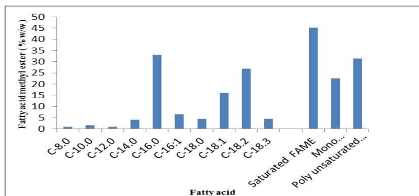
Fig.5 Fatty acid composition of Chlorella sp.
