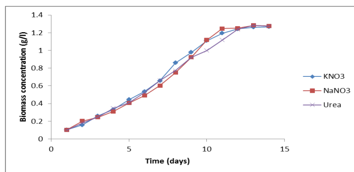
Fig.1. Dry weight of Chlorella sp. under different nitrogen sources
