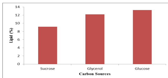
Fig.4. Lipid content of Chlorella sp. under different carbon sources
