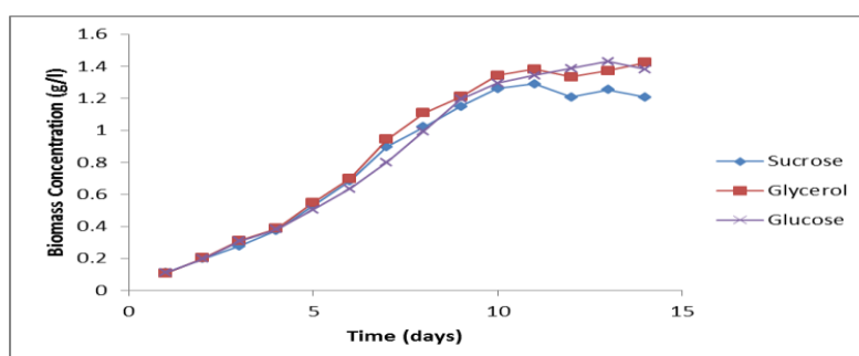
Fig.3. Dry weight of Chlorella sp. under different organic carbon sources
