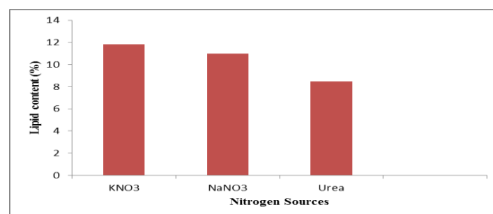
Fig.2. Lipid content of Chlorella sp. under different nitrogen sources
